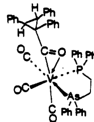
Figure 4. Representation of the coordination in the \eta^2 -acyl compound (arphos)V(CO) 3 ( \eta^2 -C 3 H 5 H 3 CO).
