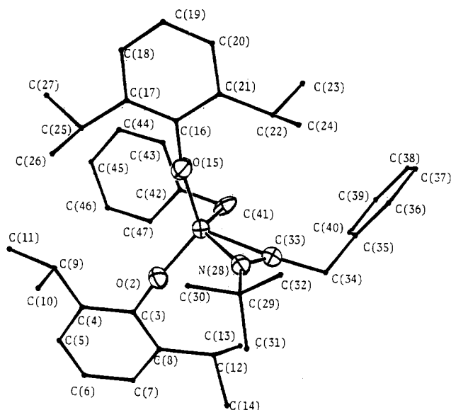
Figure 1. ORTEP view of \text{Ti}(\text{OAr-2,6-Pr}^i)_2(\eta^2\text{-Bu}^t\text{NCCH}_2\text{Ph})\text{-(CH}_2\text{Ph)} (OAr-2,6-Pr i = 2,6-diisopropyl phenoxide).
