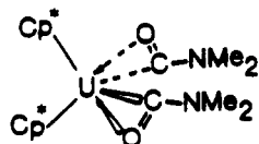
Figure 8. Coordination environment in the bis( \eta^2 -carbamoyl) \text{Cp}^*_2\text{U}(\eta^2\text{-Me}_2\text{NCO})_2 .
