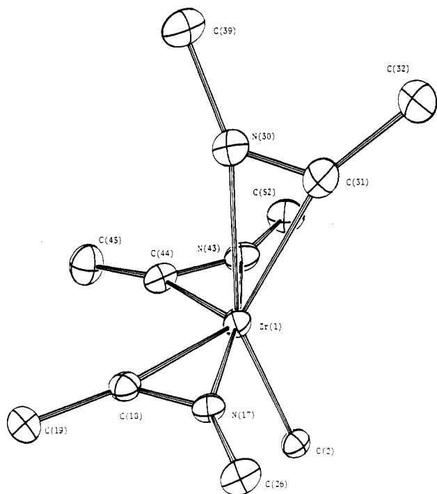
Figure 3. ORTEP view of the central coordination environment in Zr(OAr-2,6-Bu 2 )( \eta^2 -Bu + NCCH 2 Ph) 3 .
