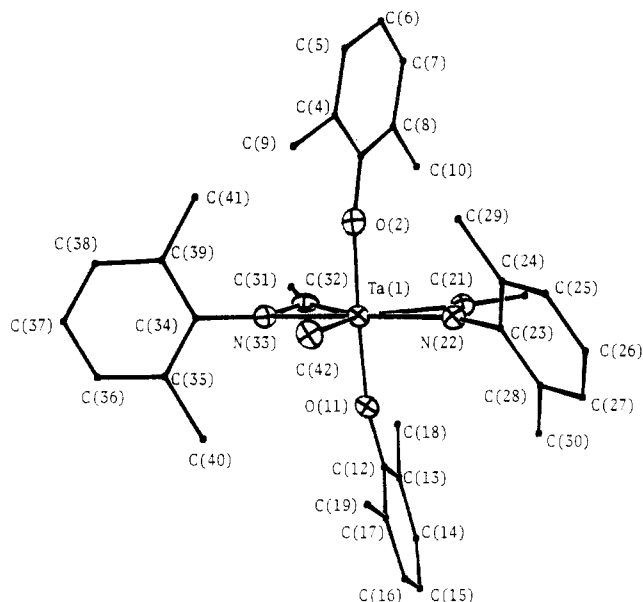
Figure 5. ORTEP view of \text{Ta}(\text{OAr-2,6-Me}_2)_2(\eta^2\text{-(xy)NCMe})_2(\text{Me}) ( \text{xy} = 2,6-dimethylphenyl).
