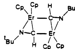
Figure 7. [\text{Cp}_2\text{Er}(\eta^2\text{-HCNCBu}^t)]_2 .
